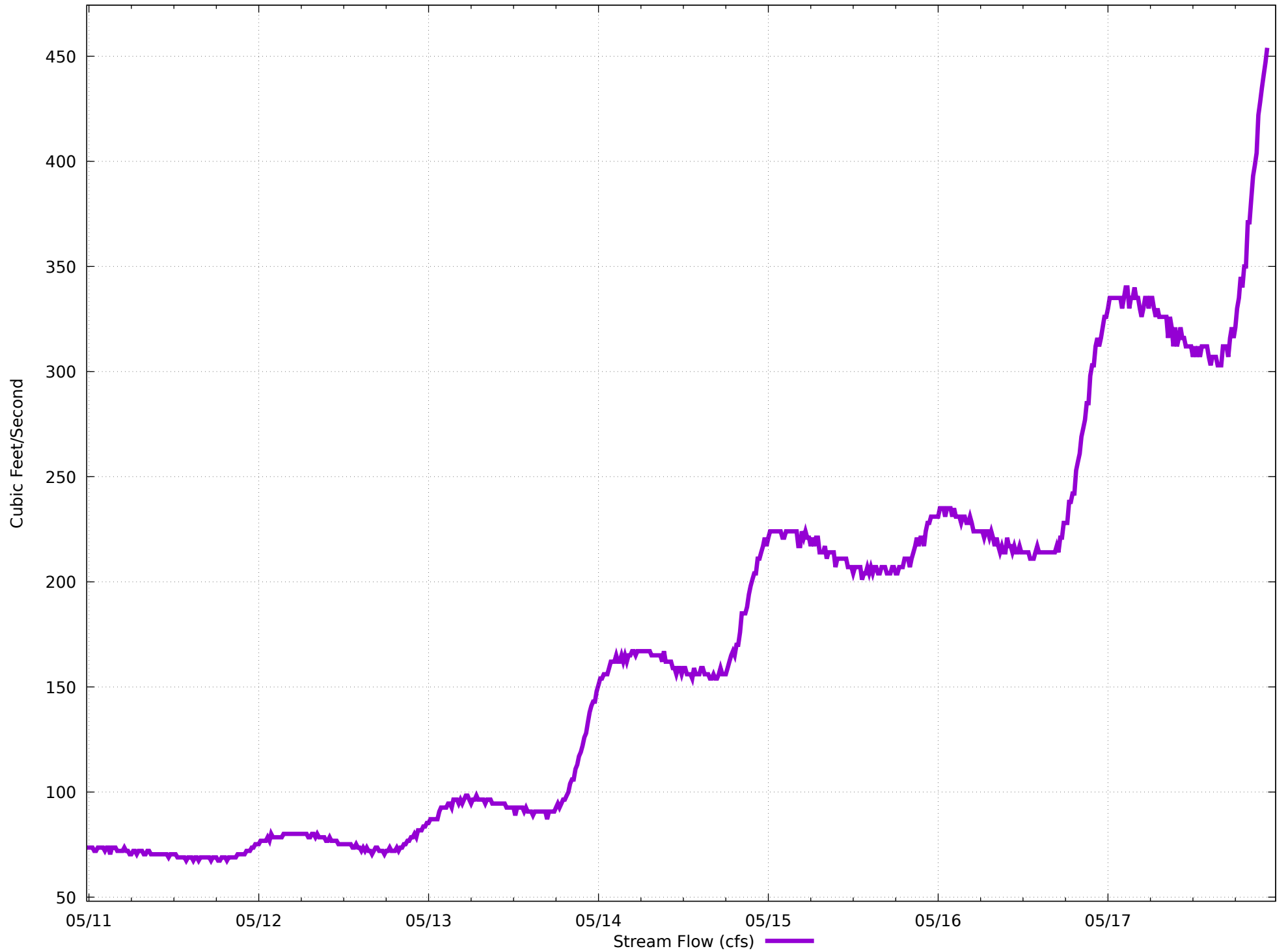
Uinta River Near Neola Gauging Station (USGS)
