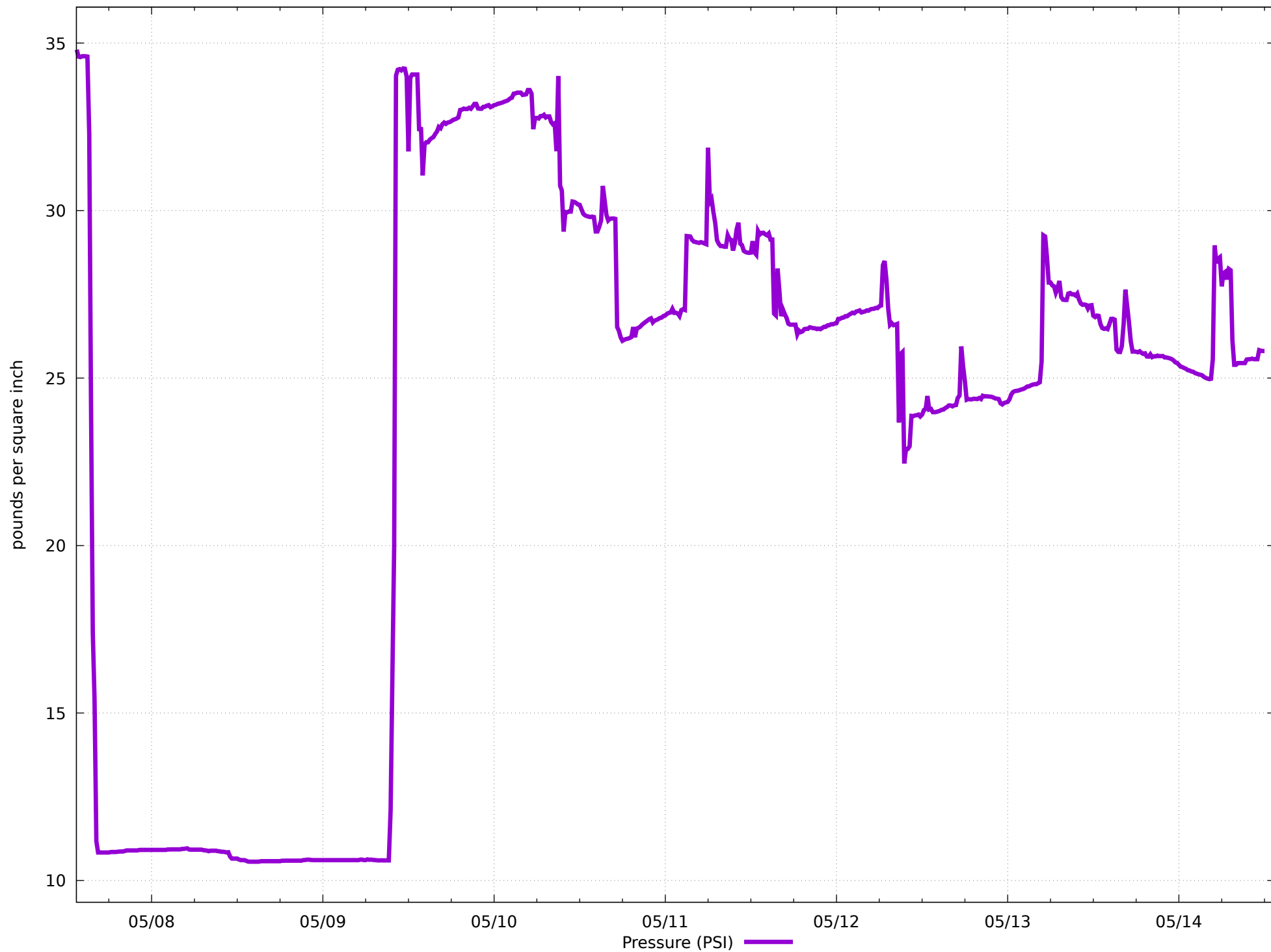
Brough Jumper Pump
